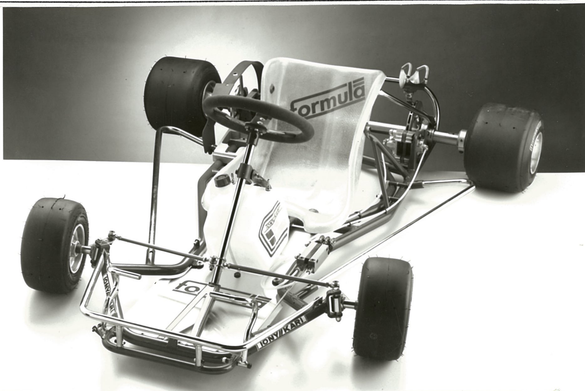
Chassis picture with tyres
